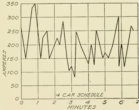
Fig. 141. Load Diagram for Small System
